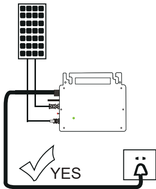
Connection diagram
