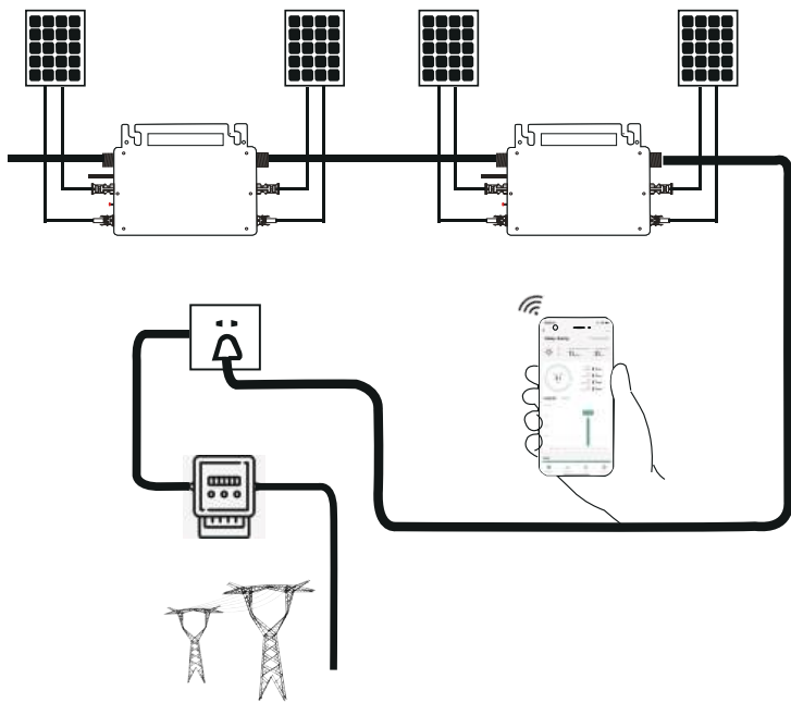
Connection diagram
